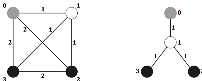
Figure 2: An example of the problem with n = 4 and p = 1 . The original transportation network G is shown on the left hand side, where gray vertex represents vertex 0, white vertex belongs to S , and black vertices belong to U . The critical transportation network is shown on the right hand side.
